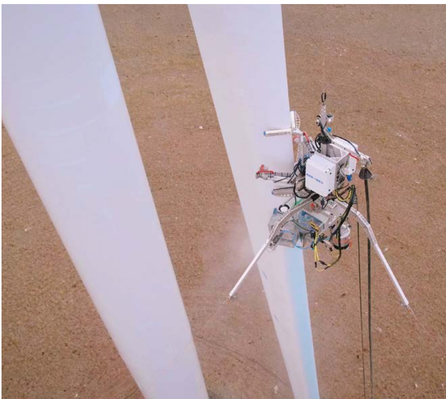
An Aeronex robot applying NEINICE to a turbine tower.
