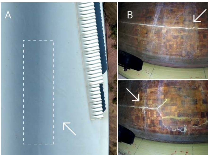
In the first photo, a drone detected a suspicious shadow on the outside of the blade. After thorough internal inspection, a severe 8-meter-long, category 5 crack was revealed, posing the risk of significant damage
