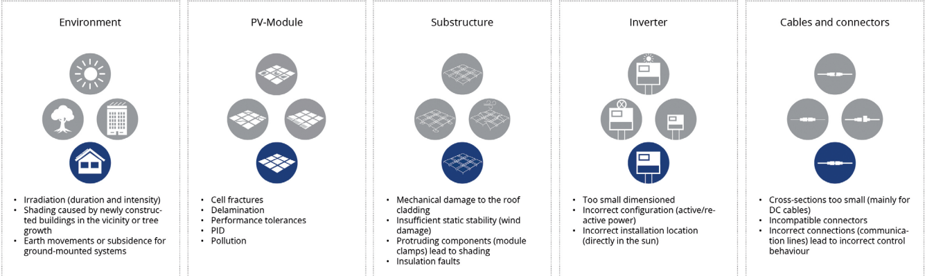
We can substantiate these diverse influences with direct examples, for this we use the CPN method (Cost-Priority-Number, financial influence on the system yield): Module - Delamination à 3.59 EUR/kWp, Inverter - Overttemperature à 1.64 EUR/kWp, Cabling - Different connector types à 0.39 EUR/kWp
