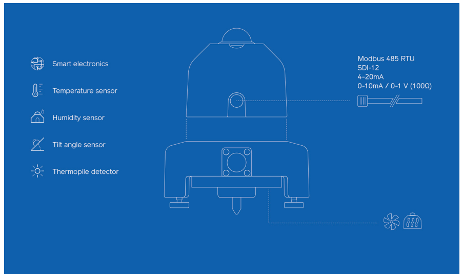
Illustration of MS-80S Class A Pyranometer with MV-01 All-Weather Heater & Ventilator
