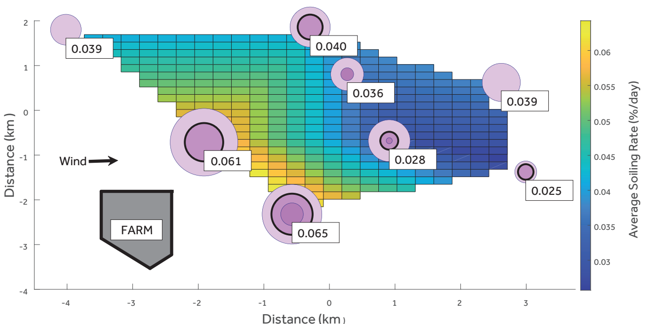
Variation of soiling rates measured by 8 soiling sensors, distributed within a utility-scale solar power plant. Multi-year average daily soiling rates in %/day, shown in text and by circle radius in figure, are highest near the edge of the plant immediately down-wind of a farm. Soiling rates could be up to 2x the averages, as shown by the outer circles at each sensor location.
